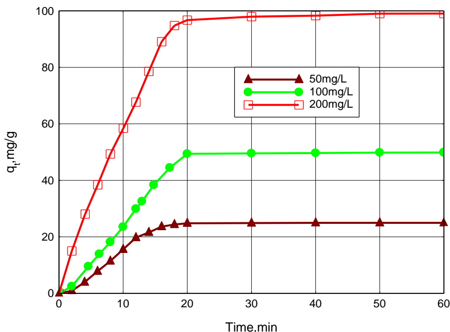
Fig. 4: Effect of time on the adsorption of ClO 4 - on MRH (Weight of the adsorbent = 0.1g, agitation speed =100 rpm, contact time = 60 min, temperature = 40°C)
