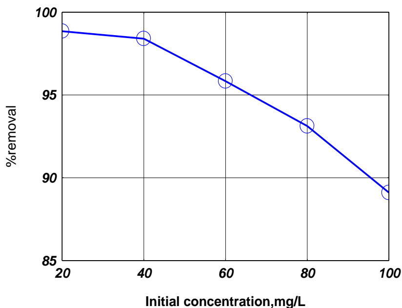
Fig. 5: Effect of initial concentration on the adsorption of ClO 4 - on MRH (Weight of the adsorbent =1g, agitation speed =100 rpm, contact time = 60 minutes, temperature =25°C)
