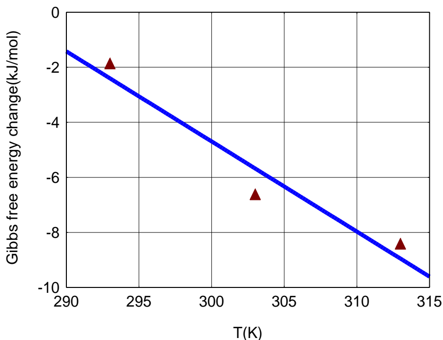
Fig. 13: Gibbs free energy variation with temperature
