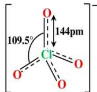
Fig. 1: Structure of perchlorate ion
